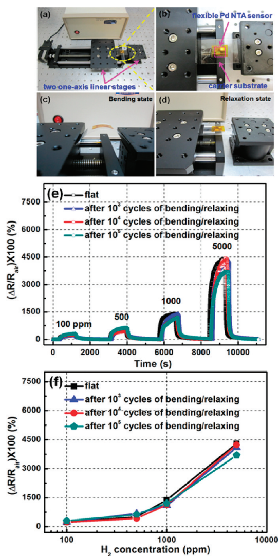
Figure 8. Mechanical robustness of a flexible Pd nanotube sensor under a cyclic bending condition: (a–d) experimental setup for fatigue test; (e,f) real-time response ( S = (\Delta R/R_{\text{air}}) \times 100 ) vs time and response ( S ) vs \text{H}_2 concentration under various \text{H}_2 concentrations (100–5,000 ppm) after repeated bending between \rho = 10.0 mm and \rho = \infty by 10^3 – 10^5 cycles.
